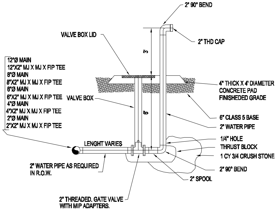
BLOW OFF DETAIL
